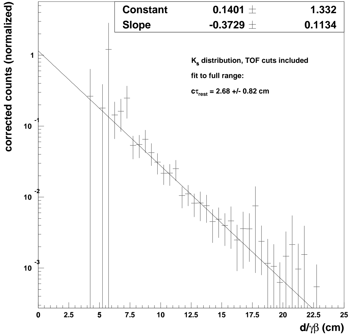
K_s (TOF cuts included) from 9,447,838 central events
