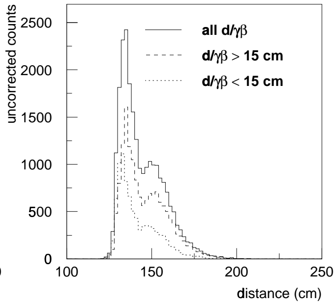
\Lambda hyperons, TOF cuts included, no corrections
