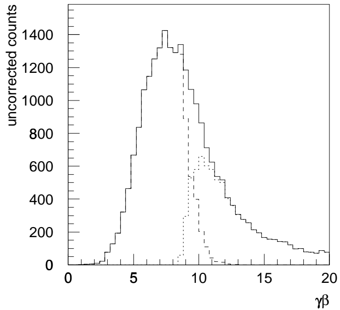
\Lambda hyperons, TOF cuts included, no corrections
