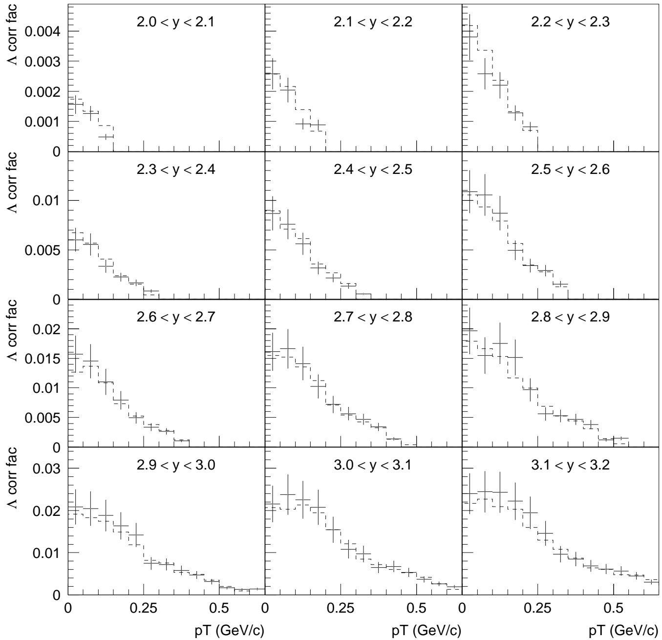
\Lambda corr. factors -- solid: Rice (no TOF cuts); dotted: S. Kelly (UCLA)
