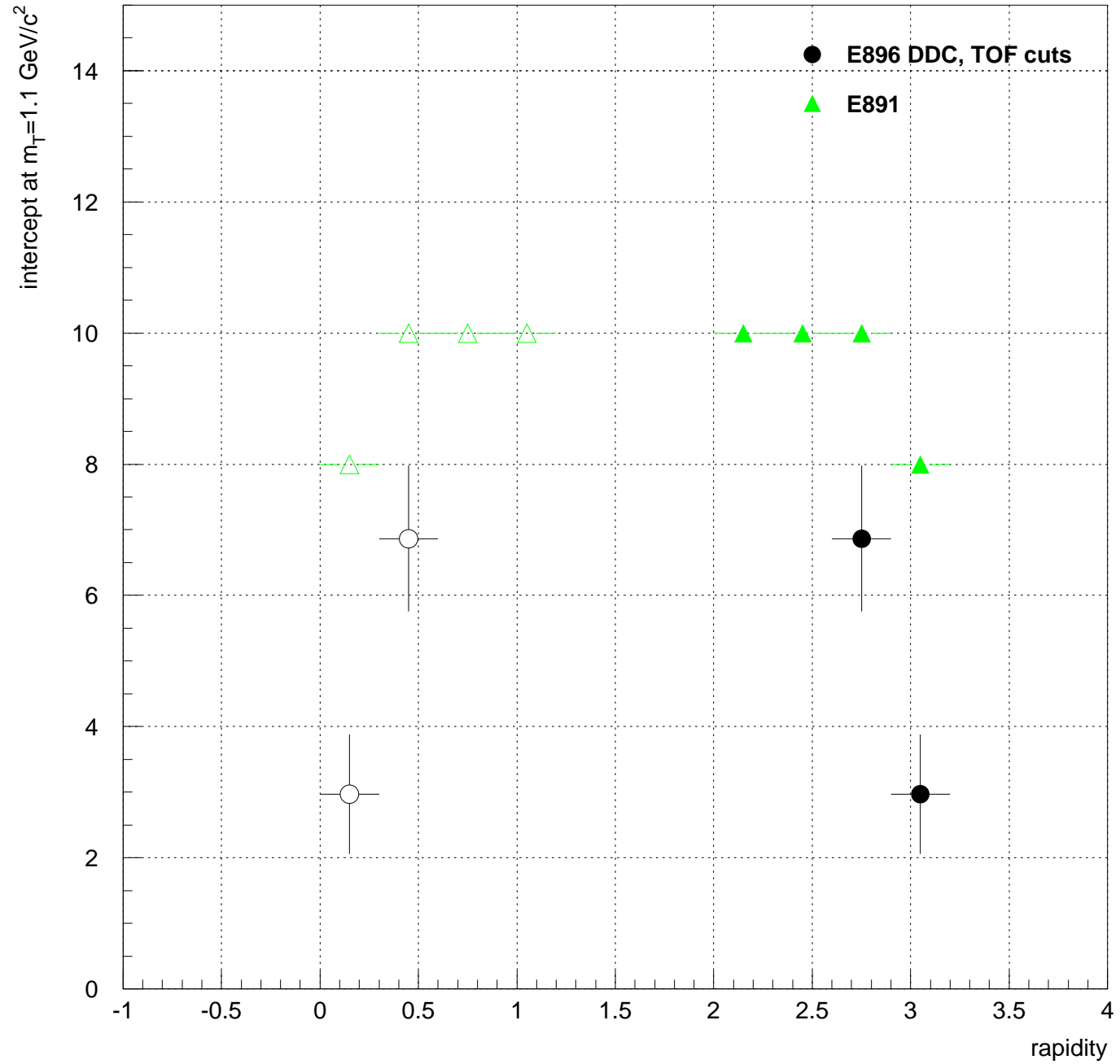
\Delta (1/N_{ev})(d^2N/dyd(p_T^2)) intercept (at m_T=1.1 \text{ GeV}/c^2 ) vs. rapidity
