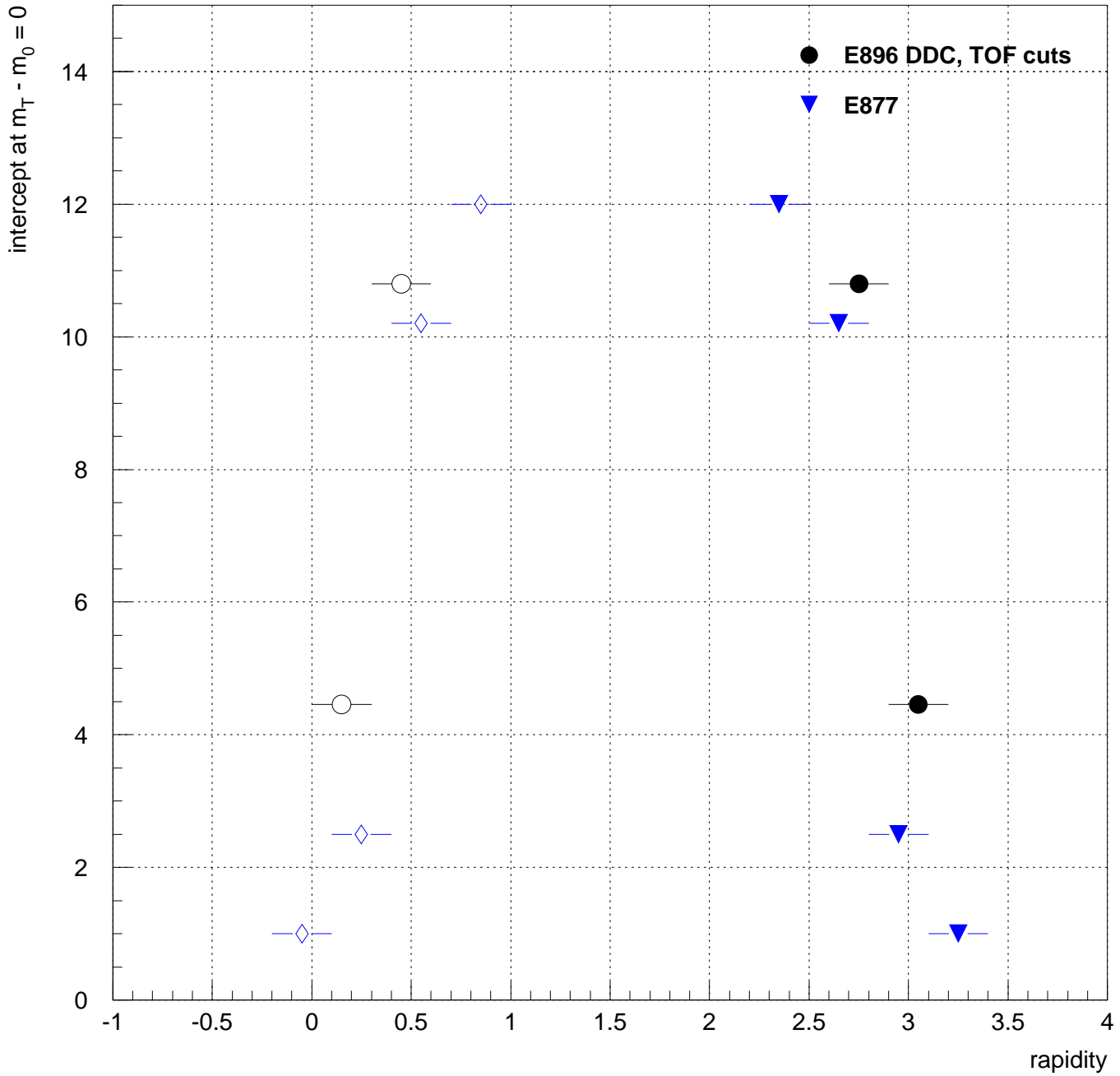
\Lambda (1/m_T^2 N_{ev})(d^2N/dm_T dy) intercept vs. rapidity
