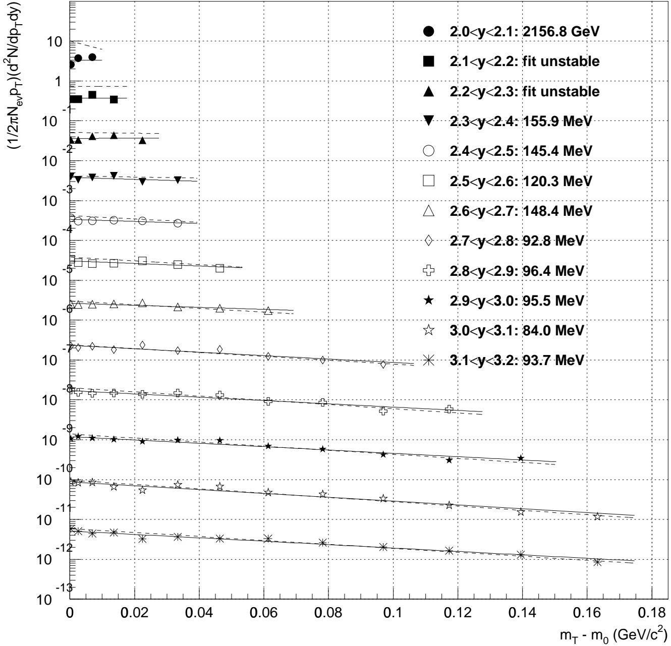
Corrected \Lambda from 113 Pass II files -- all geo, kine cuts, TOF cuts incl
