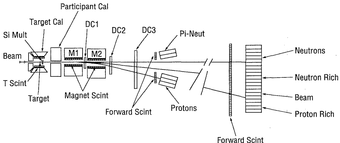
FIG. 2. E814 experimental setup. M1 and M2 are dipole magnets. DC1, DC2, and DC3 are drift chambers used to track particles in the forward spectrometer. Solid lines in the figure represent trajectories for neutral particles, beamlike particles (with Z/A = \frac{1}{2} ) and protons with 14.6 GeV/c momentum.
