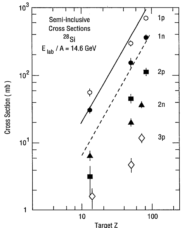
FIG. 3. Semi-inclusive cross sections for few nucleon removal from ^{28}\text{Si} . The error bars indicate statistical uncertainties. The solid line and the dashed line represent results from calculations where the virtual photon spectrum is folded with experimental \sigma(\gamma, p) and \sigma(\gamma, n) cross sections, respectively.
