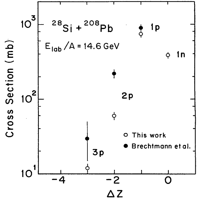
FIG. 7. Semi-inclusive electromagnetic cross sections obtained in this work (blank circles) compared to those from Ref. 8 (solid circles) plotted as function of units of charge removal.
