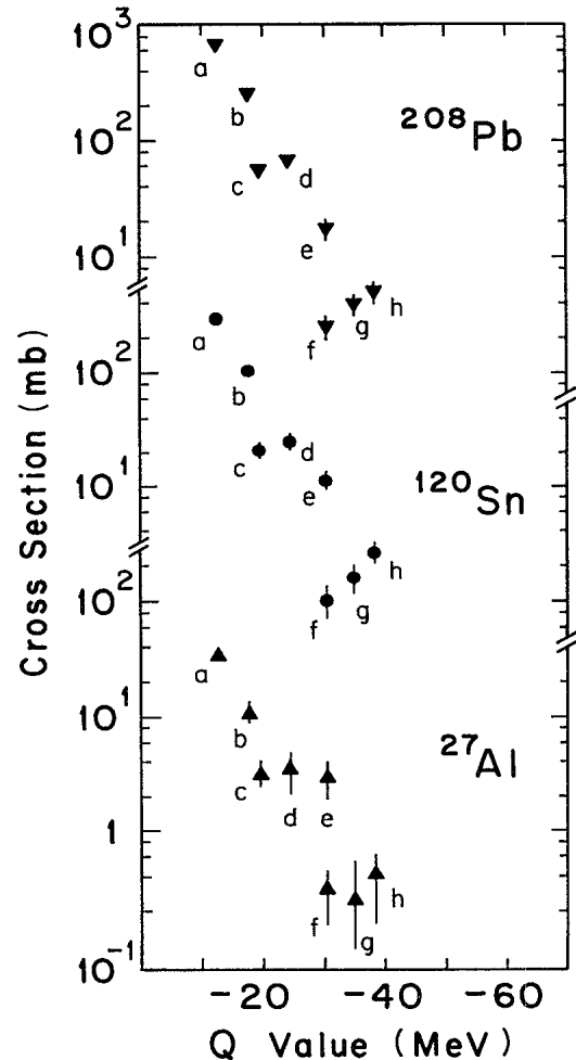
FIG. 6. Cross sections for electromagnetic dissociation as functions of the Q value of the decay channel. Experimental data are grouped according to target type. The label associated with each experimental point indicates a different dissociation channel: (a) 1p + ^{27}\text{Al} , (b) 1n + ^{27}\text{Si} , (c) 2p + ^{26}\text{Mg} , (d) 1n1p + ^{26}\text{Al} , (e) 2n1p + ^{25}\text{Mg} , (f) 2n + ^{26}\text{Si} , (g) 2n2p + ^{24}\text{Mg} , and (h) 2n1p + ^{25}\text{Al} .
