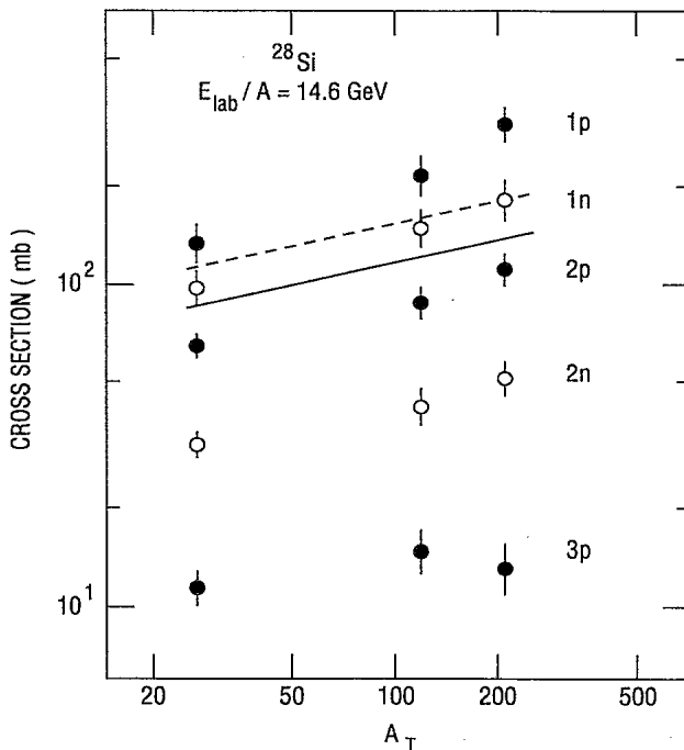
FIG. 4. Semi-inclusive hadronic cross sections for few nucleon removal from ^{28}\text{Si} . The dashed line represents results from the limiting fragmentation model from Ref. 8. The solid line represents results from the geometrical model from Ref. 14.
