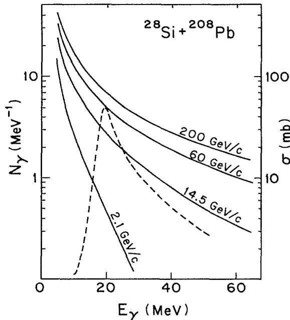
FIG. 1. Virtual photon spectrum for ^{28}\text{Si} + ^{208}\text{Pb} for different beam momenta (left-hand scale) superimposed on the cross section (right-hand scale) for real photon absorption by the ^{28}\text{Si} nucleus.
