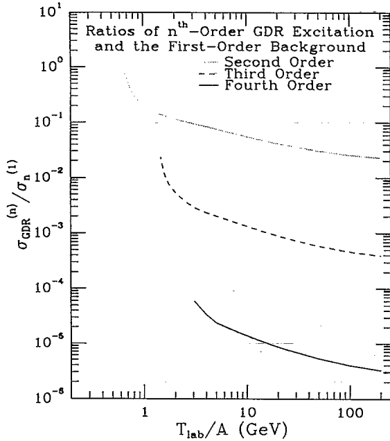
FIG. 7. The ratios of the n th-order GDR cross section, \sigma_{\text{GDR}}^{(n)} and the integral of the total first-order cross section over the same excitation energy range, \sigma_n^{(1)} , as a function of projectile kinetic energy.
