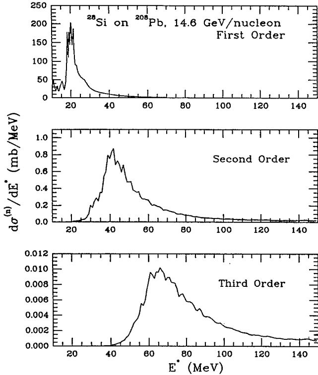
FIG. 3. The total differential Coulomb excitation cross sections for ^{28}\text{Si} on ^{208}\text{Pb} at E_{\text{lab}}/A=14.6 GeV for the first-, second-, and third-order processes.
