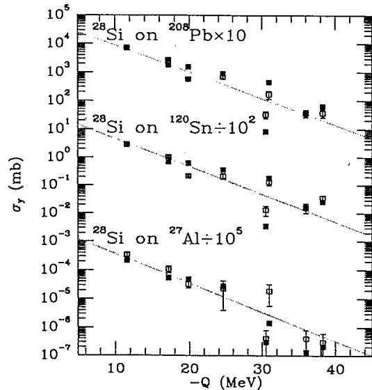
FIG. 9. Comparison of E814 data, Ref. 10, for the electromagnetic dissociation of ^{28}\text{Si} at E_{\text{lab}}/A = 14.6 GeV/nucleon (open squares with error bars), and the present calculation (solid squares) for all measured decay channels and targets. The dotted line is a pure exponential and is included to guide the eye.
