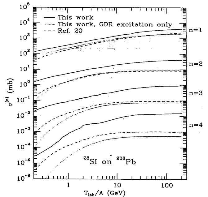
FIG. 5. The total excitation cross sections from the schematic method (Ref. 20, dashed line), and from this work (solid line), as a function of the projectile kinetic energy. Also shown, the total cross sections by integration over only the GDR (dotted line).
