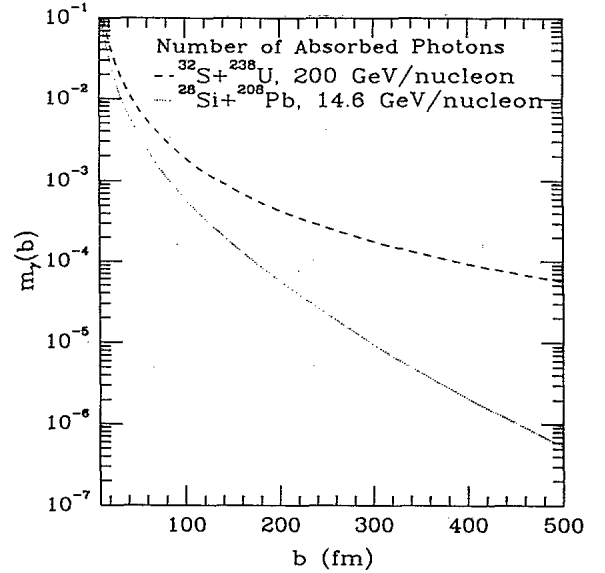
FIG. 2. The mean number m_\gamma of absorbed photons for collisions with impact parameter b .
