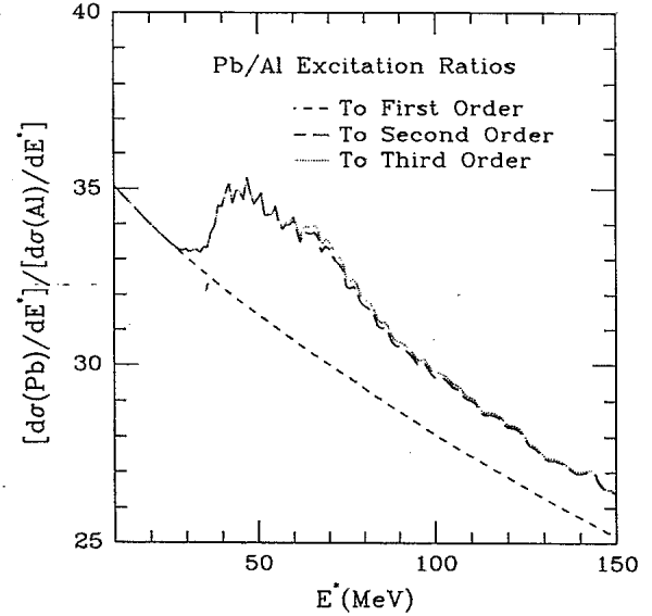
FIG. 4. The ratio of the differential Coulomb excitation cross sections for ^{28}\text{Si} on ^{27}\text{Al} and ^{208}\text{Pb} targets as a function of the excitation energy.
