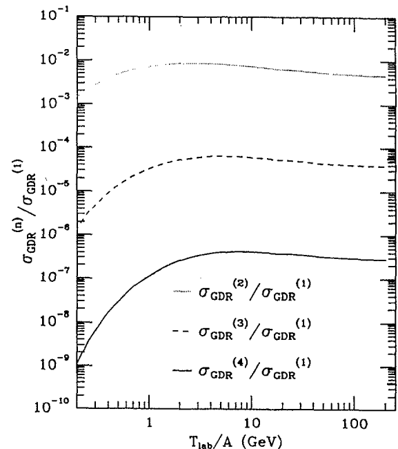
FIG. 6. The ratios of the n th-order GDR excitation cross sections to the first-order GDR cross section as a function of the projectile kinetic energy.
