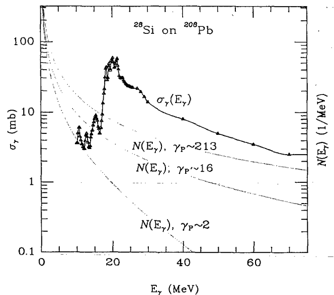
FIG. 1. The photoabsorption cross section from Ref. 25 for a ^{28}\text{Si} projectile and the integrated virtual photon spectrum of a ^{208}\text{Pb} target moving with Bevalac, AGS, and SPS energies through the rest frame of the projectile.
