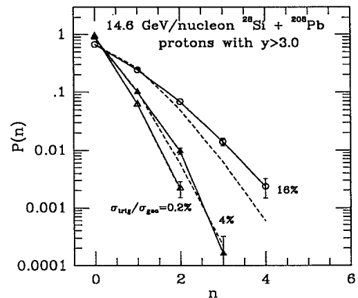
FIG. 6. Probability distribution to find n protons per event for three different levels of centrality obtained by triggering on the TCAL. Data points are connected by solid lines. Also shown as dashed lines are Poisson distributions with the same mean as data.
