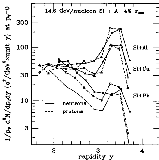
FIG. 9. Rapidity density at p_t=0 of protons (open symbols and dashed lines) and neutrons (full symbols and solid lines) for Si + Al, Cu, and Pb (circles, triangles, and squares, respectively). For clarity of the picture, neutron points are displayed 0.02 unit of y above the center of each rapidity bin, protons points 0.02 unit below. The data points are connected to guide the eye. Systematic errors dominate and are estimated to be less than 15% (see text). Dotted line: from a simulation using HIJET with rescattering [17] for protons from Si + Pb collisions.
