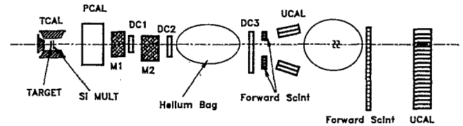
FIG. 1. Schematic outline of the E814 experimental setup in 1989.
