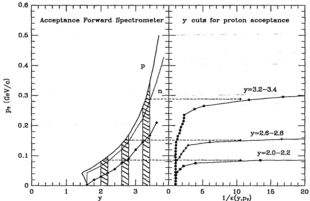
FIG. 2. Left: Acceptance in a p_t vs y plot for protons and neutrons (solid and dotted lines, respectively). The solid line with diamonds marks the p_t values, where the acceptance drops below 100%. Right: Acceptance correction factors for three selected rapidity bins, indicated as hatched areas in left panel, as a function of p_t for protons.
