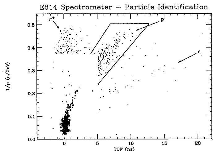
FIG. 3. Particle identification plot of inverse momentum vs time-of-flight difference with respect to a speed of light particle for charge 1 particles from events satisfying any of the three second level E_t triggers.
