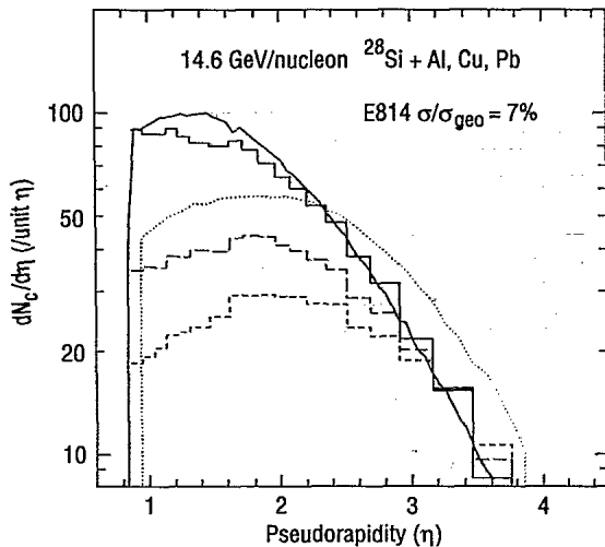
FIG. 11. dN_c/d\eta for the upper 7% of the geometric cross section of each of the targets. The dotted curve is from a HIJET calculation that does not contain rescattering while the solid line is from a HIJET calculation that does contain rescattering.
