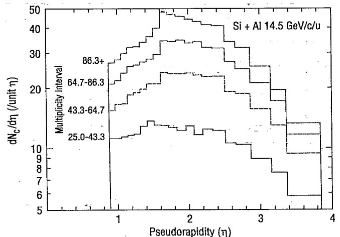
FIG. 10. dN_c/d\eta for various multiplicity cuts in the data from the Al target.
