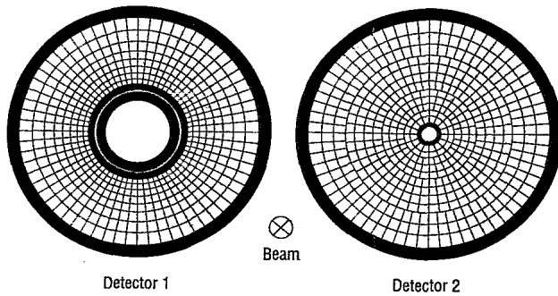
FIG. 2. Pad segmentation of the E814 silicon multiplicity detectors. Each of the detectors has 512 pads.
