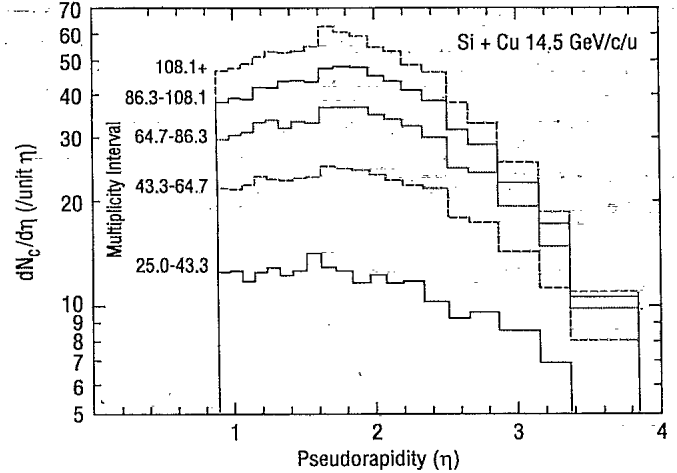
FIG. 9. dN_c/d\eta for various multiplicity cuts in the data from the Cu target.
