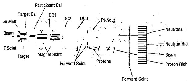
FIG. 1. Diagram of the E814 experiment. The beam enters through a hole in the back wall of the target calorimeter. Forward going particles pass through the participant calorimeter opening and magnets M1 and M2 which provide the deflection for the forward spectrometer. Track positions are measured in drift chambers DC1, DC2, and DC3. Charge is measured in the forward scintillators and energy is measured in the U/Cu calorimeters. The drawing is not to scale.
