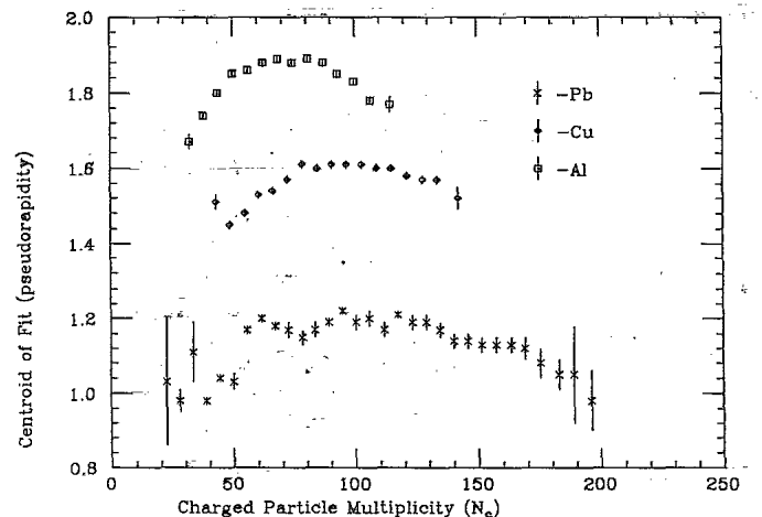
FIG. 12. Centroids of Gaussian fits to the dN_c/d\eta spectra as a function of the multiplicity of the event.
