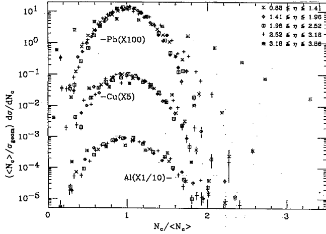
FIG. 15. Observed multiplicity distributions, plotted in KNO variables for each target at various pseudorapidity intervals. The distributions are virtually identical except for the most forward ( 3.18 \leq \eta \leq 3.86 ) interval where the distribution is wider for all three targets.
