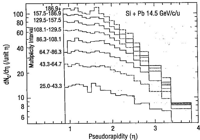
FIG. 8. dN_c/d\eta for various multiplicity cuts in the data from the Pb target.
