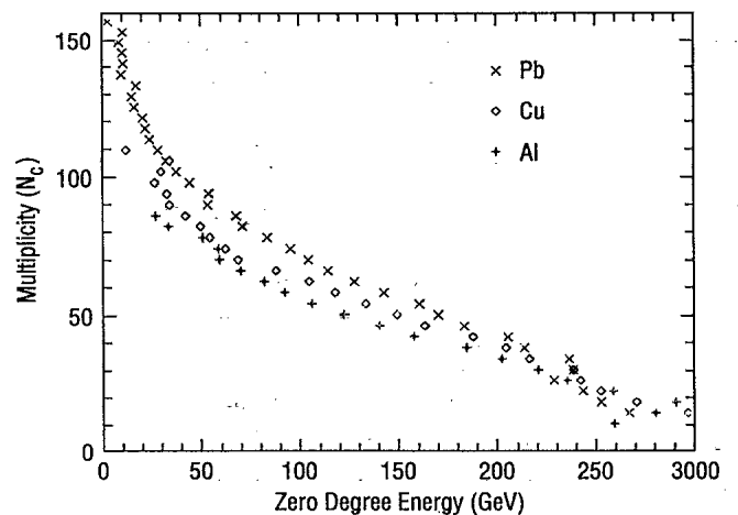
FIG. 14. Correlation between the measured charged particle multiplicity measured in the multiplicity detector and the zero-degree energy as measured by the downstream uranium calorimeters. The data were taken with an E_t trigger and the figure made by projecting on the multiplicity axis.
