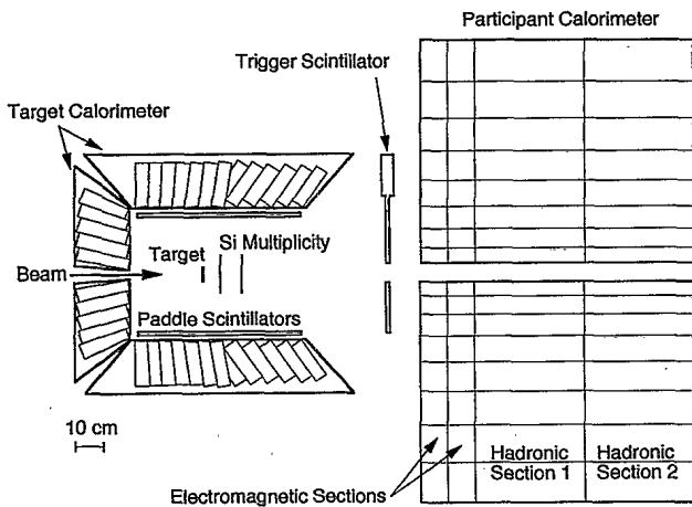
FIG. 1. Schematic diagram of the part of the E814 experimental setup used for the measurements reported in this paper.
