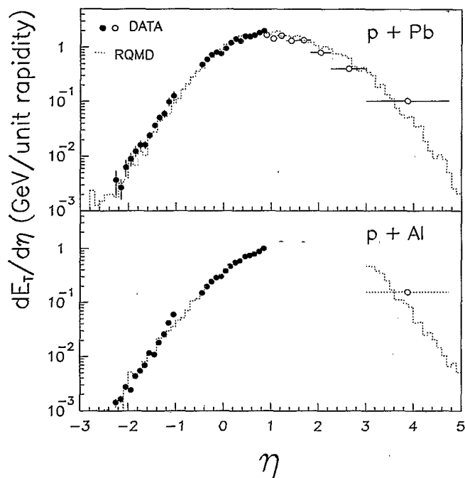
FIG. 6. Corrected dE_T/d\eta distribution for p +Pb (top) and p +Al (bottom) reactions plotted on a semilogarithmic scale to enhance the results in the tail of the distributions at low pseudorapidity.
